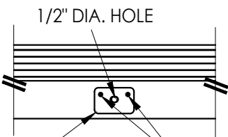
DETAIL 2 Outswing ASTRAGAL STRIKE PLATE
