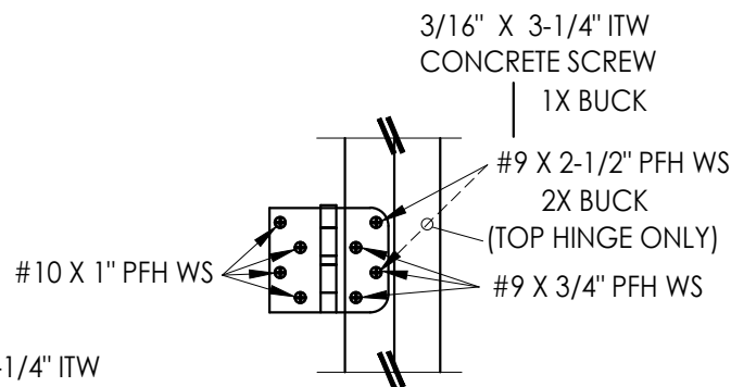
HINGE DETAIL
