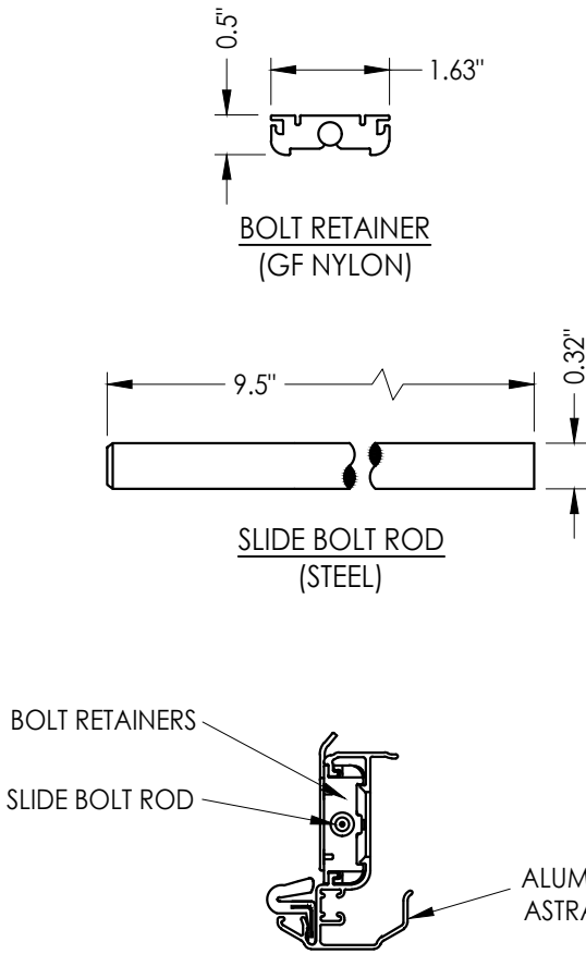
ALUMINUM ASTRAGAL ASSEMBLY
