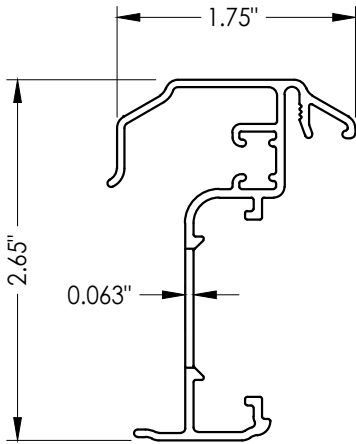
ASTRAGAL SECTION
