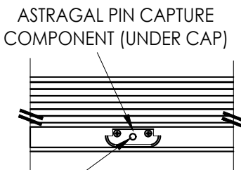
DETAIL 2 Inswing Articulating Threshold
